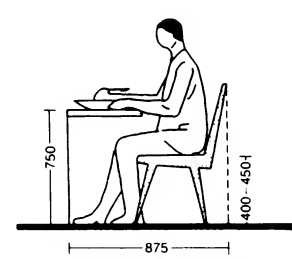
14 Dimensions: sitting and dining room chair
